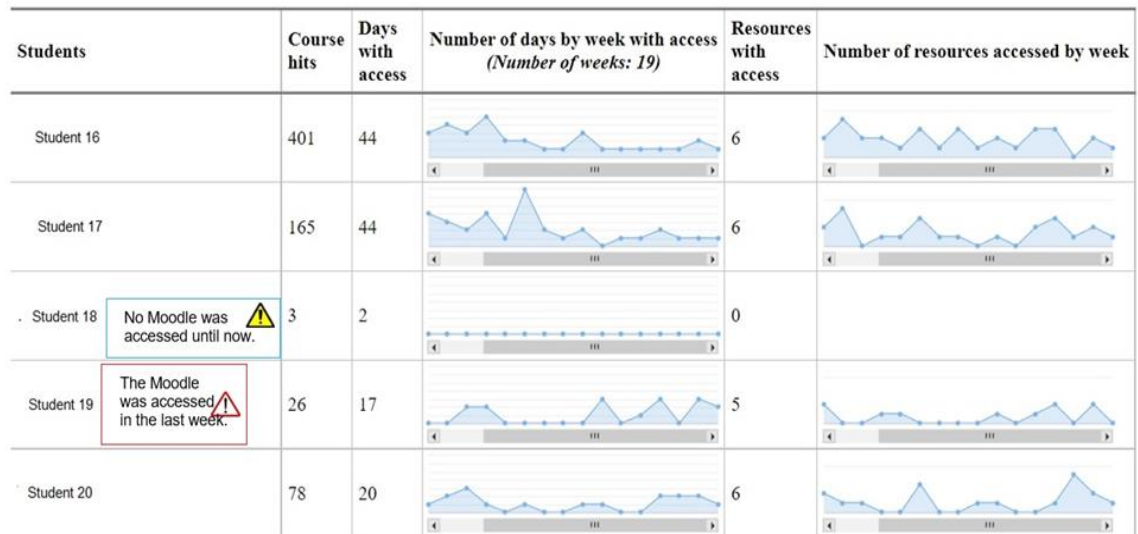
Figure 13: Group 4 Hits Distribution
