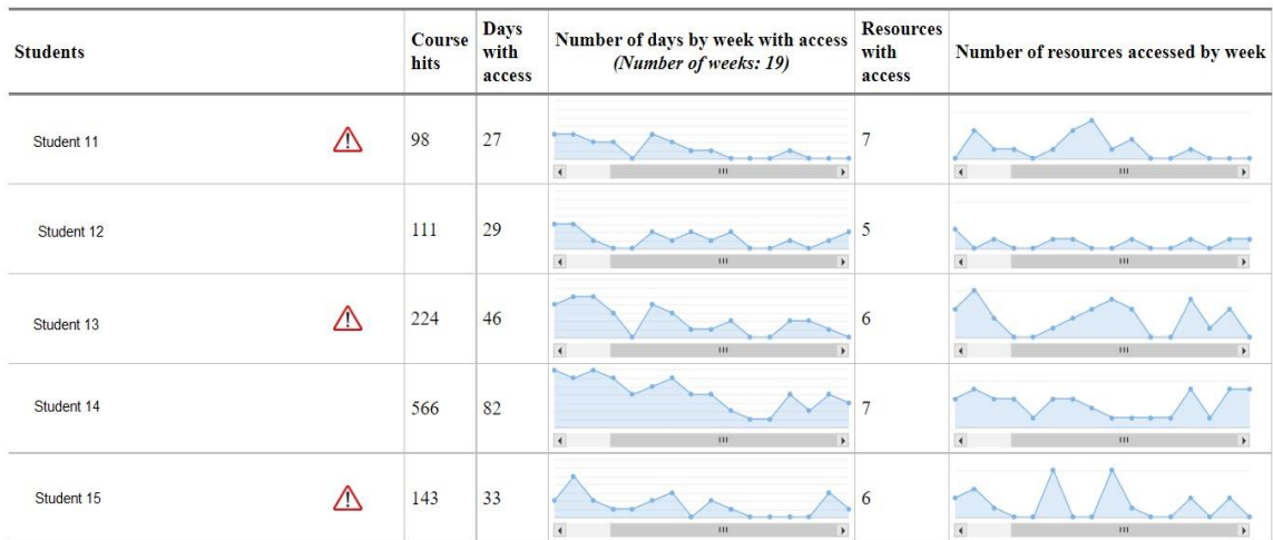
Figure 12: Group 3 Hits Distribution
