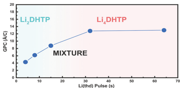
Fig. 2 GPC versus Li(thd) pulse length ( \text{H}_4 -DHTP pulse length fixed to 10 s); the resultant product ( \text{Li}_2\text{DHTP} or \text{Li}_4\text{DHTP} ) is highlighted.
