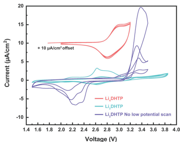
Fig. 4 Cyclic voltammograms for \text{Li}_2\text{DHTP} and \text{Li}_4\text{DHTP} films. The \text{Li}_4\text{DHTP} voltammogram is offset by 10 \mu\text{A cm}^{-2} .
