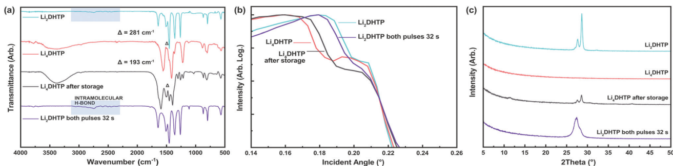
Fig. 3 Representative (a) FTIR spectra (most important spectral features highlighted), (b) XRR patterns, and (c) GIXRD patterns to show the differences between the \text{Li}_2\text{DHTP} and \text{Li}_4\text{DHTP} films.
