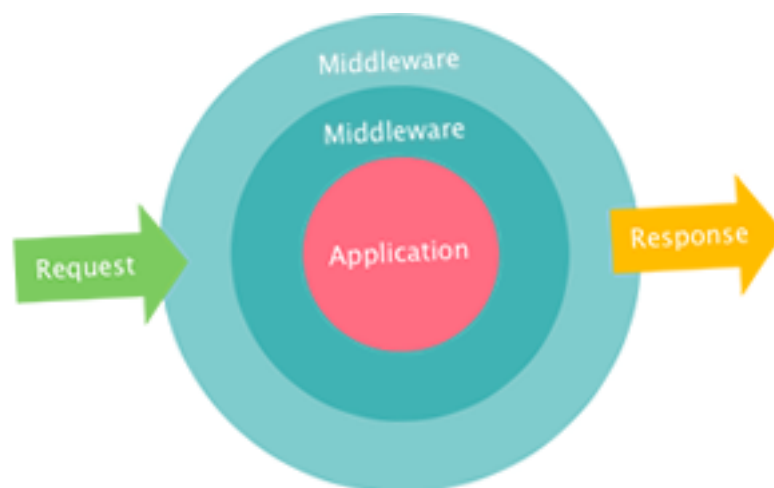
Figure 3 Middleware illustration
