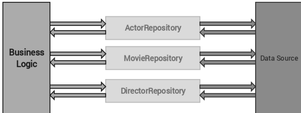
Figure 4 Repository layer
